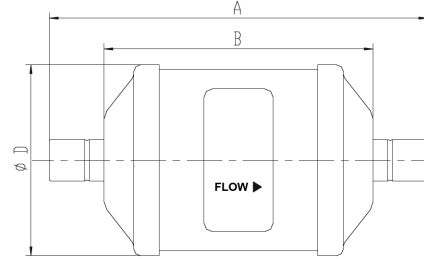
Solder Connection
